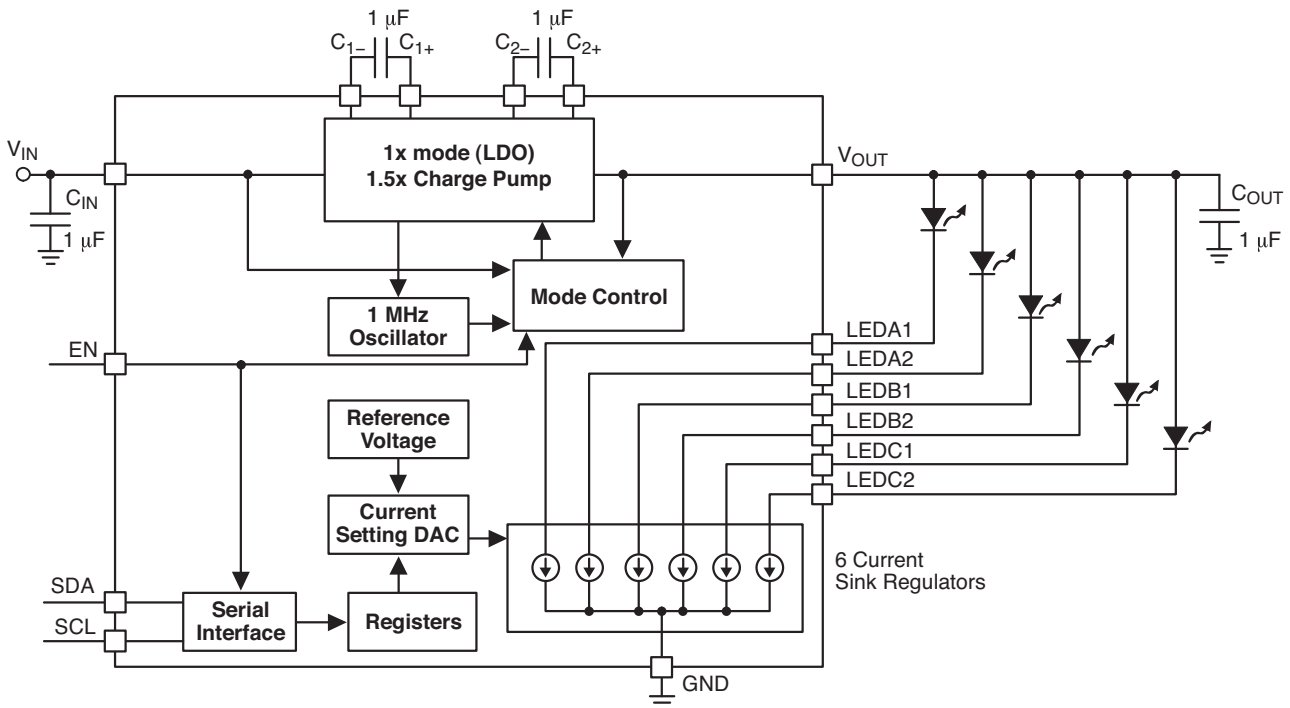
Figure 25. W-5626 Functional Block Diagram
