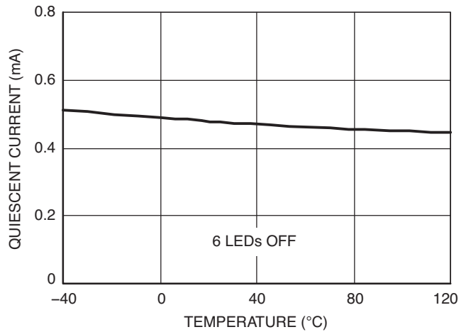
Figure 6. Quiescent Current vs. Temperature (1x Mode)
